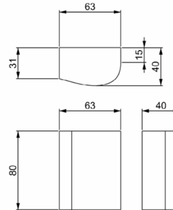
2. half end
